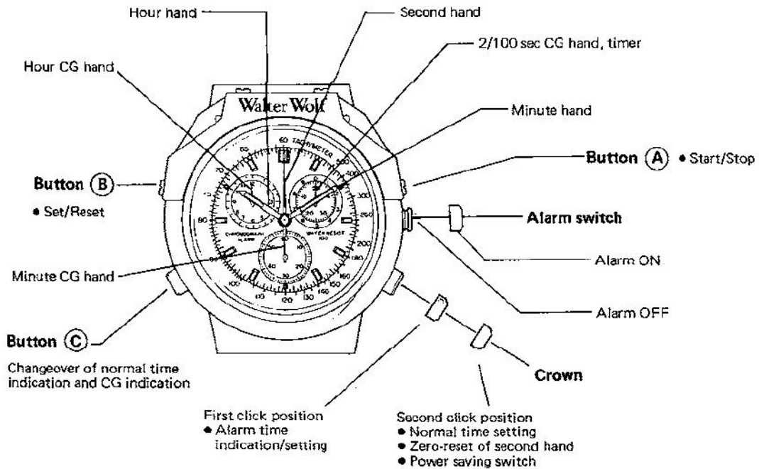
CAL. 3530/3531
