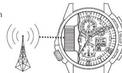
An antenna for receiving the radio signals is located inside the watch (on the 9:00 position).
