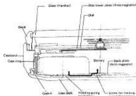
Without the battery hatch (Example: Snap type case back construction)
