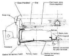
With battery hatch (Example: One-piece type case back construction)
