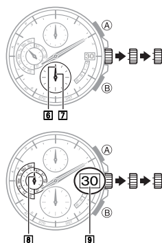
Day Indicator during home position adjustment
