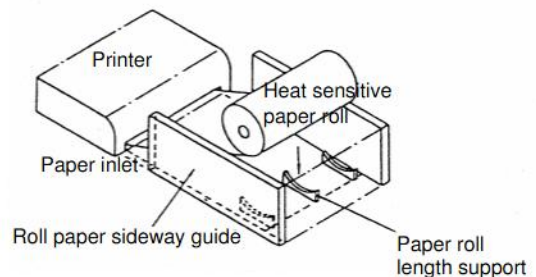
Figure 8-9 Roll without Core
