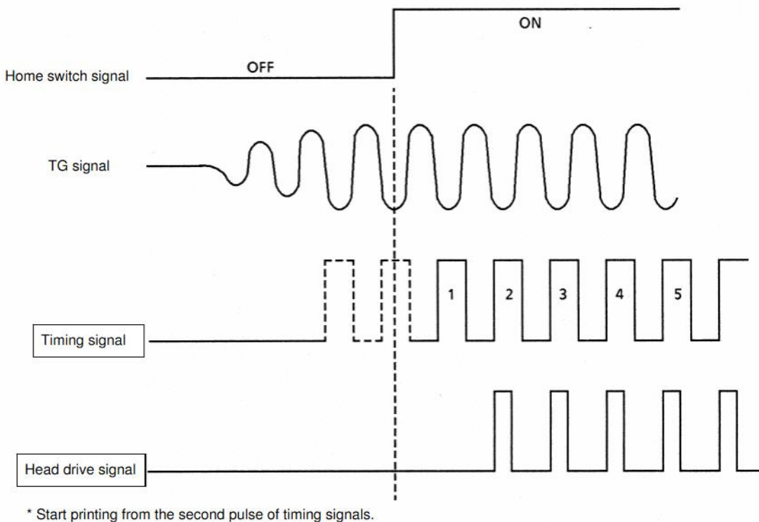
Figure 4-2 Printing Start Timing Chart
