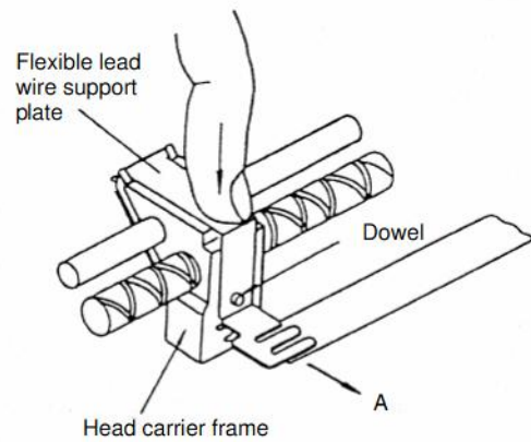
Figure 8-13 Pulling out the Flexible Cable Plate
