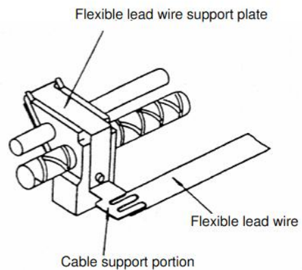
Figure 8-12 Removing the Flexible Lead Wire
