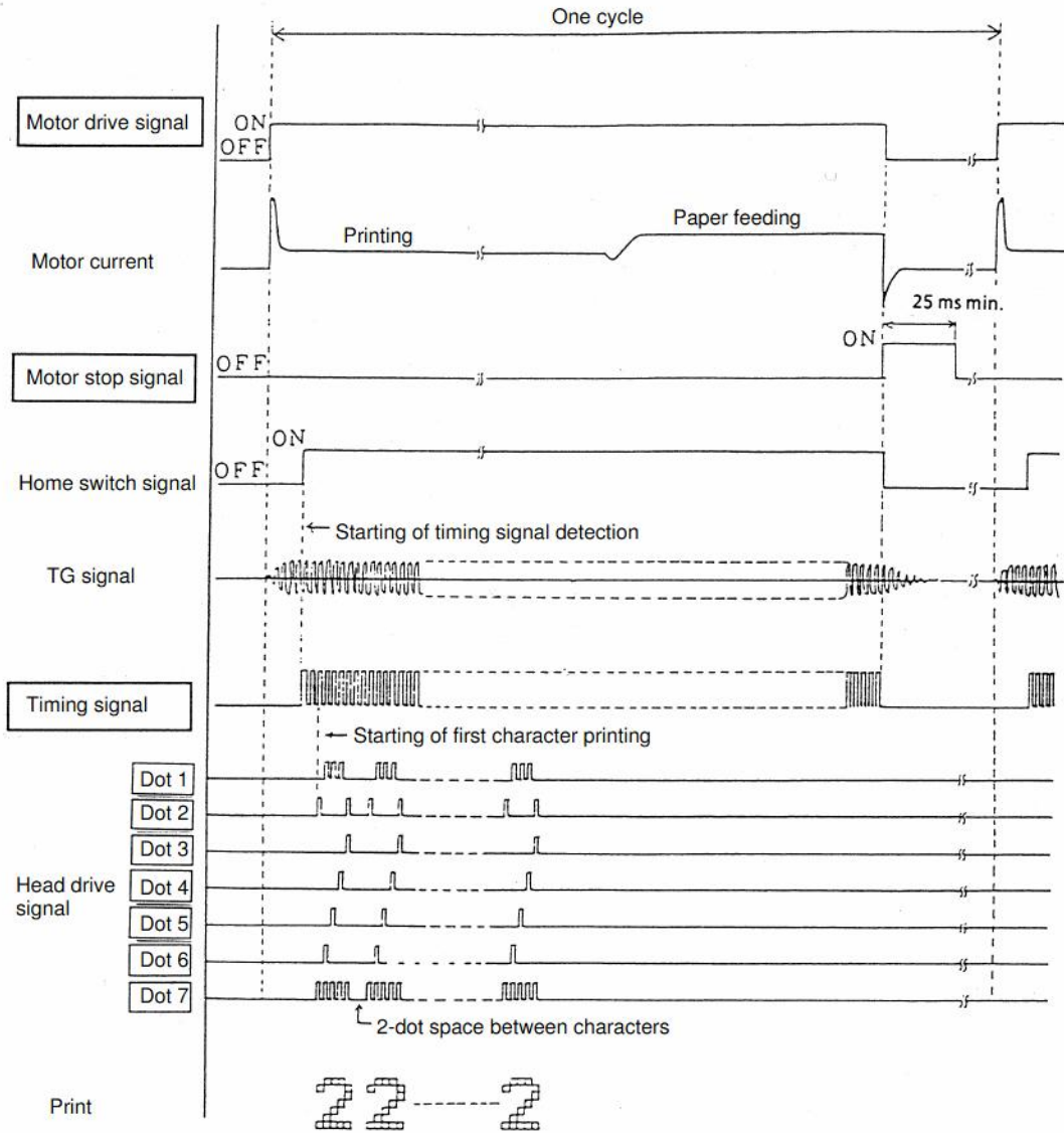
Figure 4-1 Timing Chart
