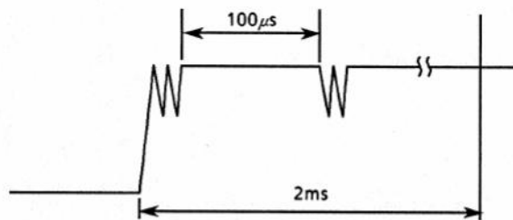
Figure 2-6 OFF-to-ON Detection
