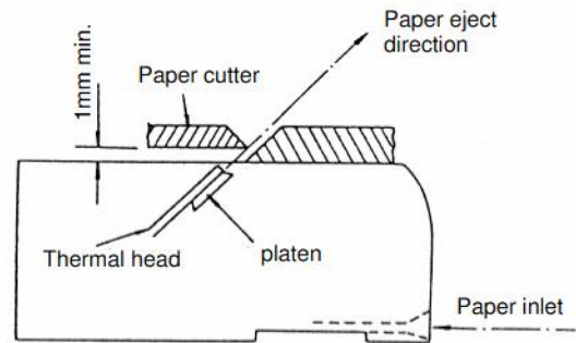
Figure 8-7 Mounting the Paper Cutter
