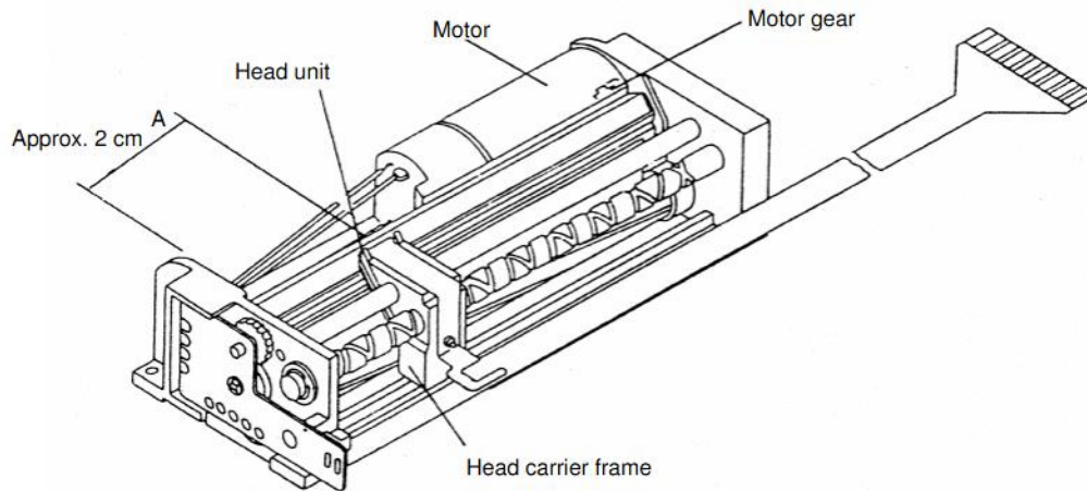
Figure 8-11 Moving the Head Carrier
