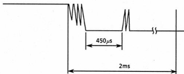
Figure 2-7 ON-to-OFF Detection
