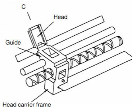
Figure 8-17 Sliding the Head along the Guide of the Head Carrier
