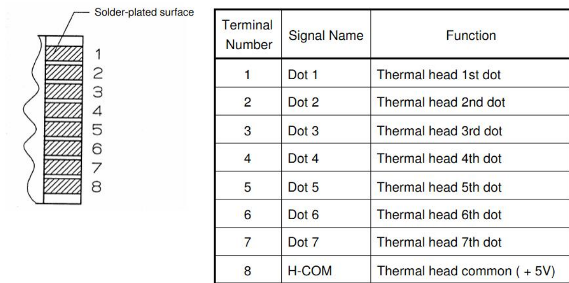
Figure 3-1 Thermal Head Control Terminal Assignment (B Head-mounted Printer)
