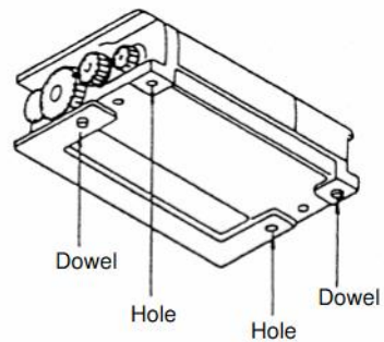
Figure 8-1 MTP102 Printer (Back)
