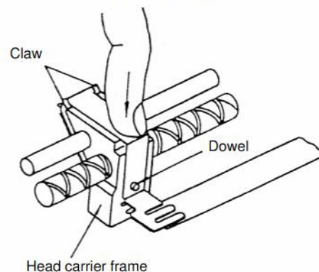
Figure 8-18 Pushing the Flexible Cable Plate
