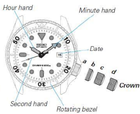
a: Screwed-in position b: Normal position c: First click d: Second click
